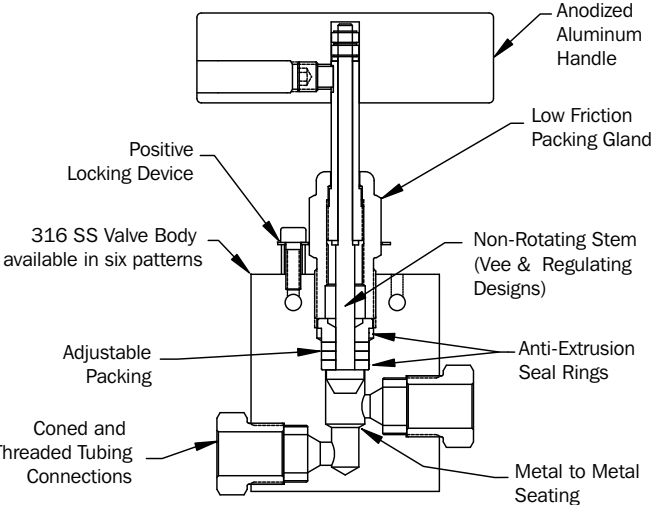
Valve Shown: 21V9M071
