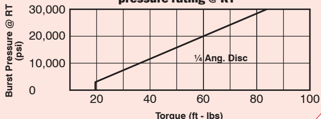
Hold-down nut torque vs. rupture disc pressure rating @ RT
